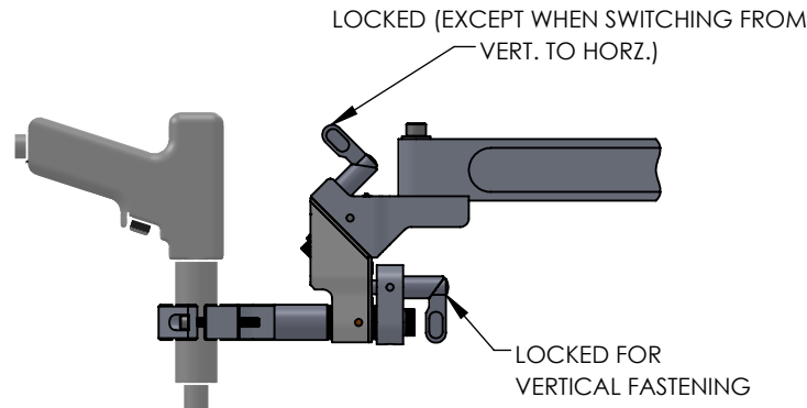
SIDE VIEW VERTICAL POSITION
